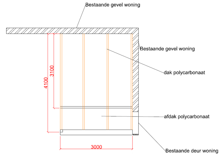
Dakenplan
