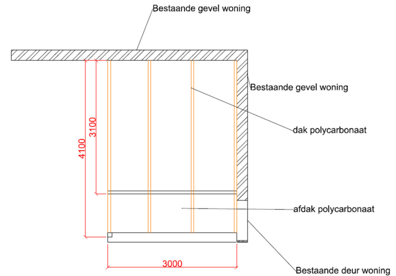
Dakenplan
